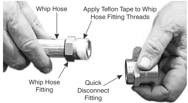
Figure 9-9. Apply Teflon Tape to Hose Fitting.
