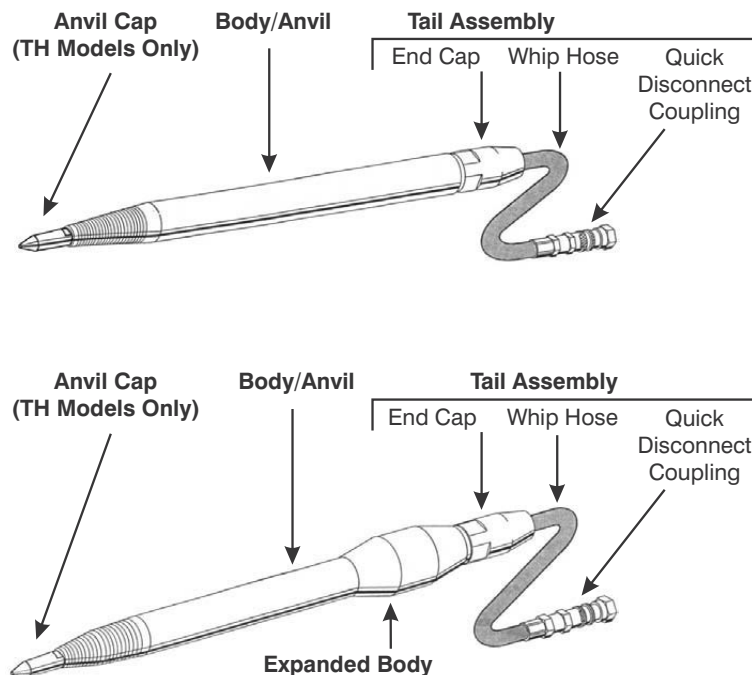
Figure 3-1.Hole-Hog Major Components
