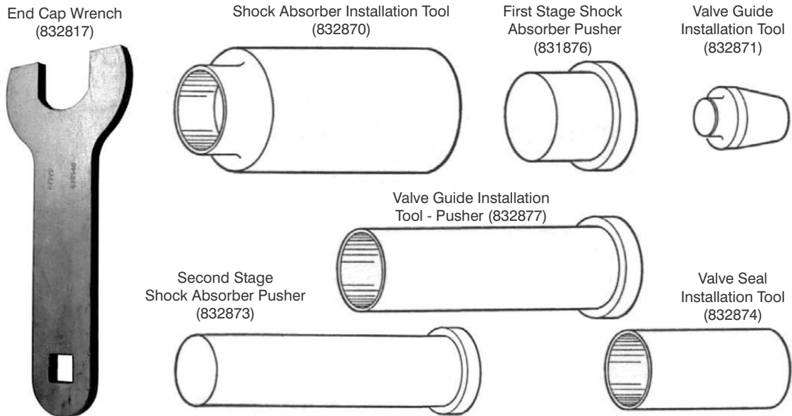
Figure 8-1. Hole-Hog Tool Kit
