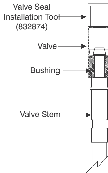
Figure 9-14. Valve Pressing Tool on Valve
