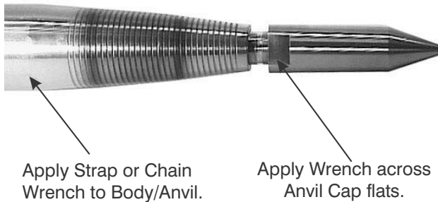
Figure 9-29. Secure Anvil Cap to Body/Anvil
